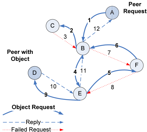
Fig. 7. A typical request sequence in Freenet.
